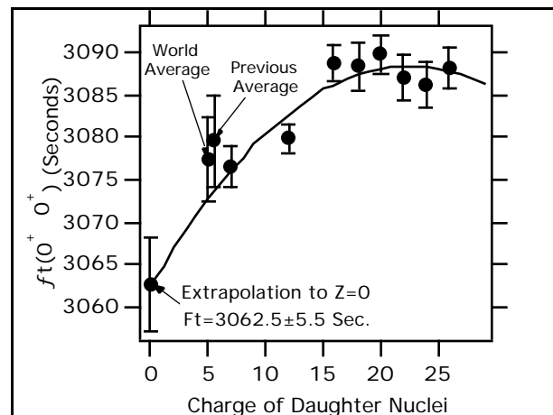
Fig. 1. The radiatively-corrected ft values for superallowed Fermi beta decays plotted against the charge of the daughter nucleus. The solid curve is a fit to the data assuming a hypothetical quadratic Z dependent isospin breaking correction proposed by Wilkinson§. Recent results from this experiment on ^{10}\text{C} , taken with previous experiments, tend to support such a dependence.
