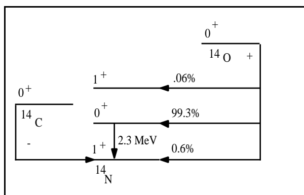
Fig. 1. The A=14 isospin triplet and decay scheme for ^{14}\text{O} decay. We will measure the spectral shape of the 0^+ \rightarrow 1^+ transition and the branching ratio of the 0^+ \rightarrow 0^+ transition.
