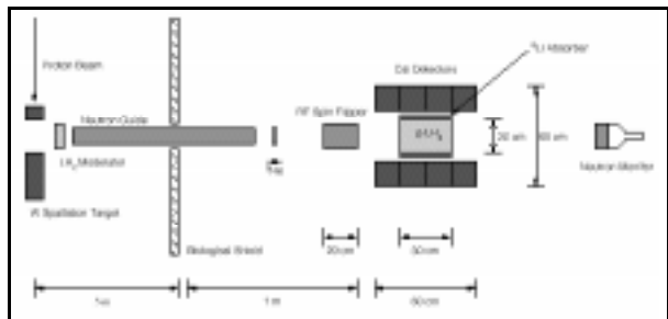
Fig. 1. Conceptual design of the proposed NPDG experiment.
