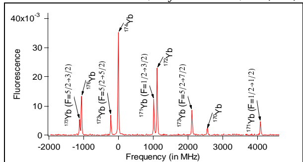
Fig.1 Laser-excitation spectrum of the 408 nm transition observed via fluorescence at 556 nm for the different isotopes and hyperfine components observed with a highly collimated atomic beam.
