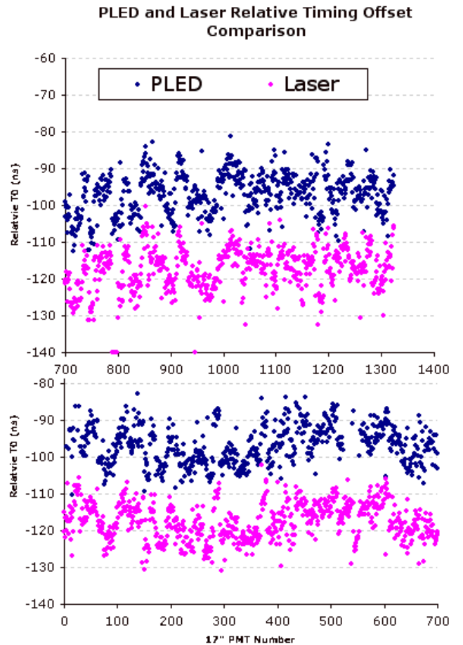
FIG. 2: Comparison of PMT relative time-offset constants deduced from the PLED and laser calibration sources. Only relative values are shown.
