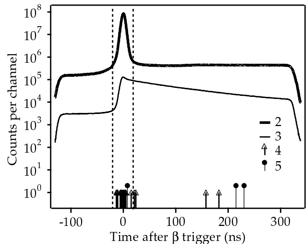
FIG. 1: Ps annihilation events as a function of time after the \beta decay ( t = 0 ). Dashed lines are at \pm 20 ns. Five-photon counts have been offset for visibility.
